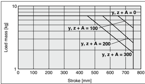
[Graph 5] Allowable load mass by stroke ø25
