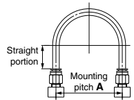
Fig. 1 Recommended piping configuration
